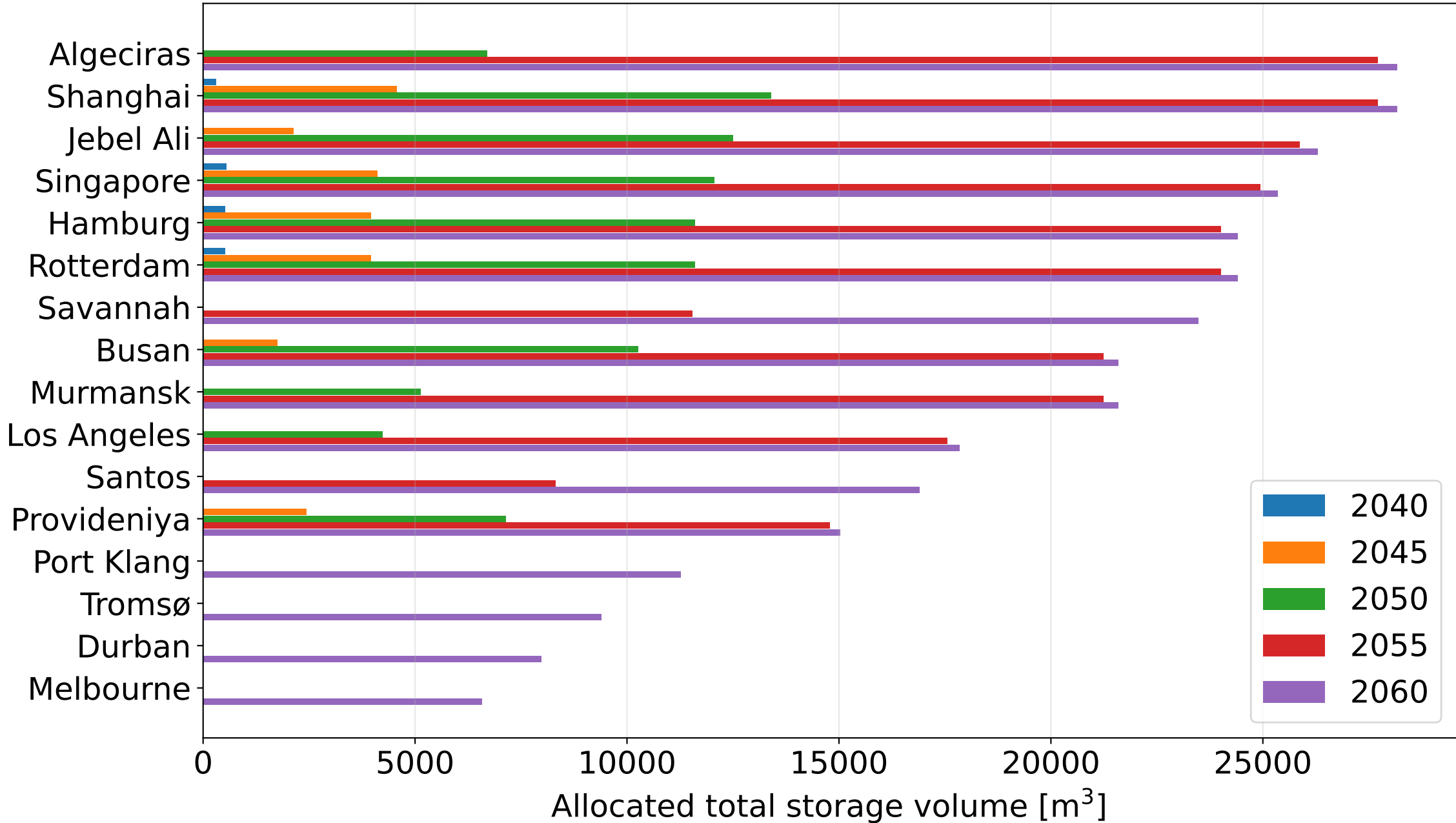
Allocated total fuel-storage volume by port
