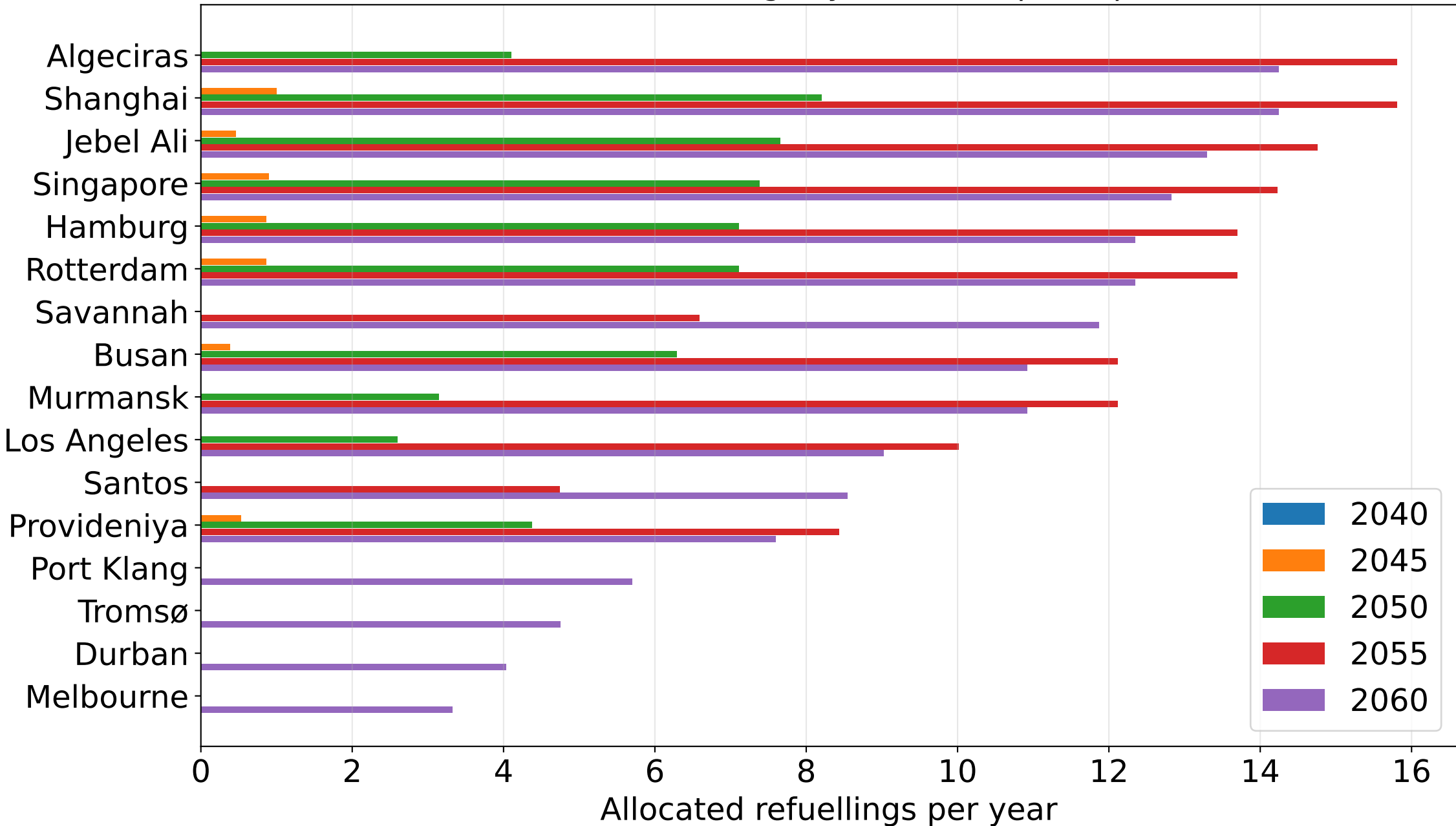
Allocated refuellings by nuclear-capable port
