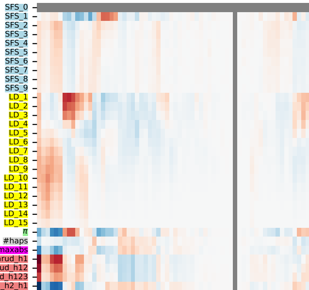
Learned Features
