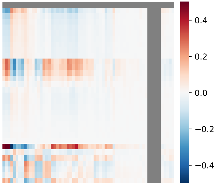
Learned Features
