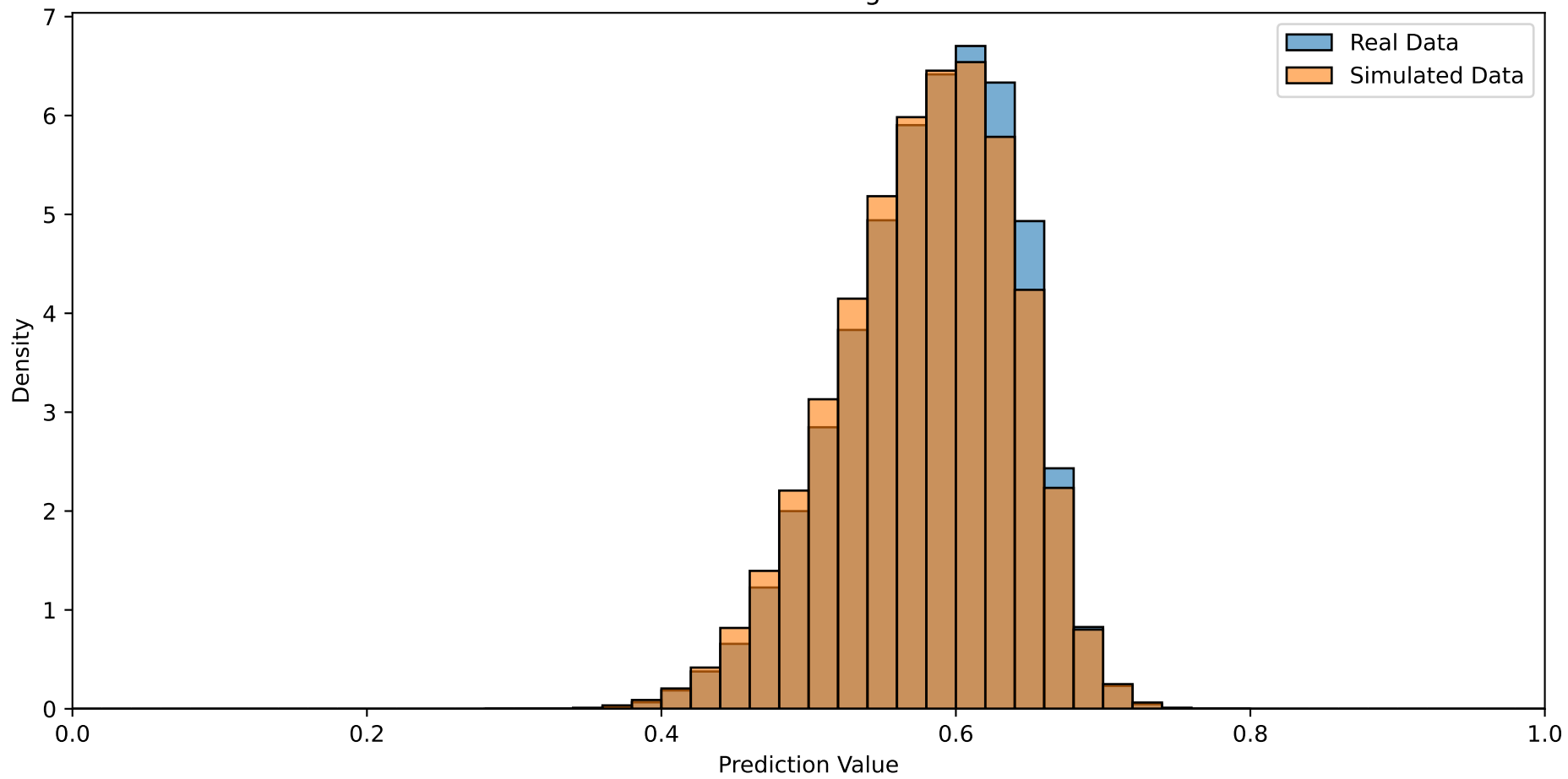
Random Weights
