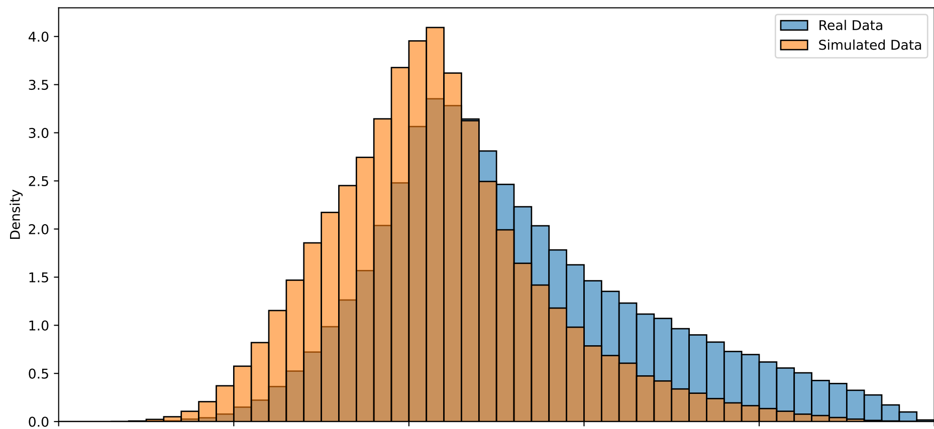
Random Weights
