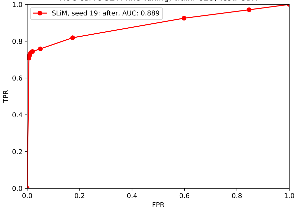
ROC curve SLiM fine-tuning, train: CEU, test: GBR
