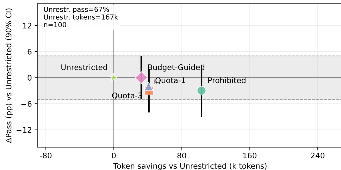
SWE-bench Verified — Claude Code
