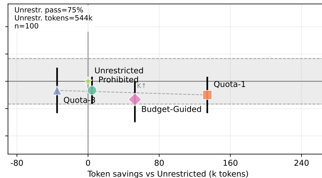
SWE-bench Verified — Codex
