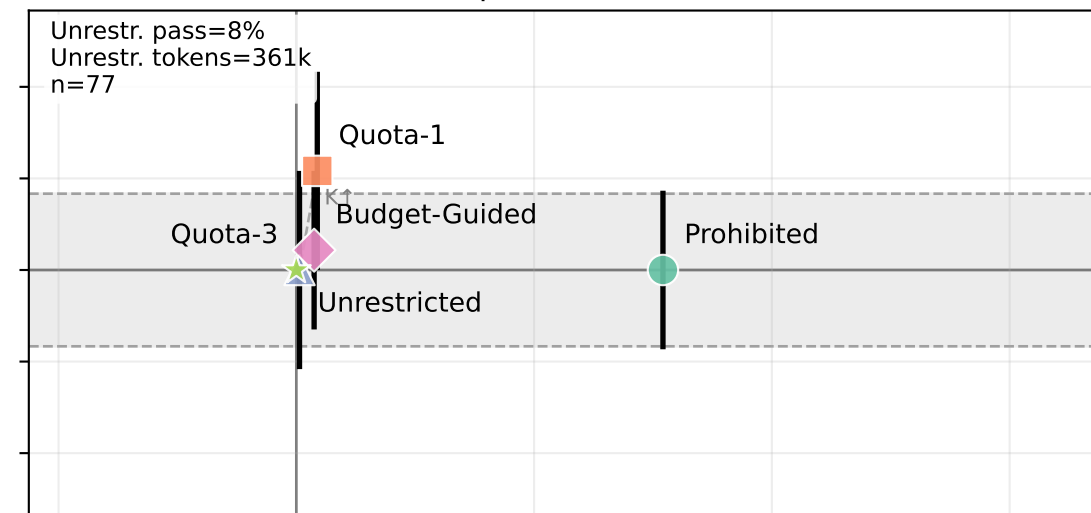
SWE-bench Lite — OpenCode (Qwen2.5-Coder-32B)
