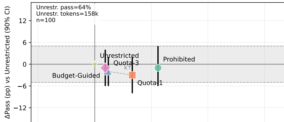
SWE-bench Lite — Claude Code
