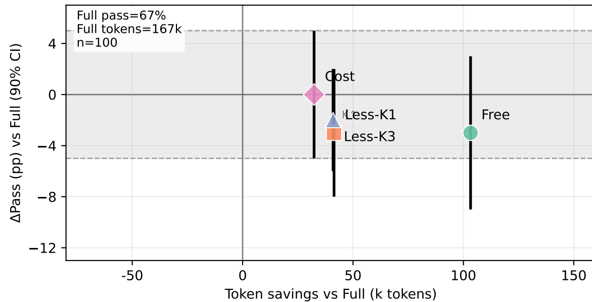
SWE-bench Verified — Claude Code
