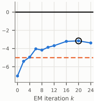
Factor model ( d = 8 )
