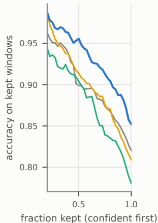
(c) Open vs closed
