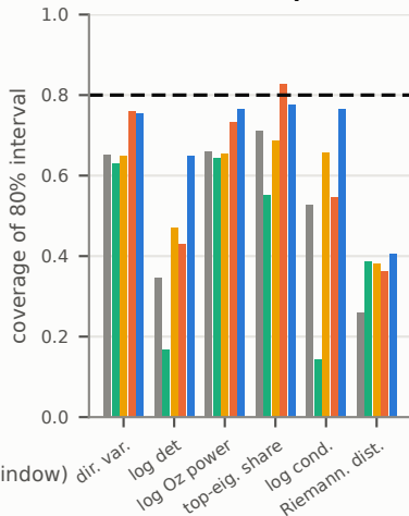
(b) Calibration, split-half
