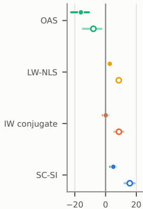
(a) Log-score gain
