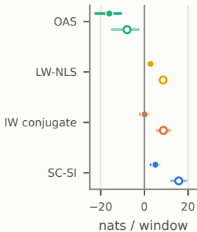
(a) Log-score gain
