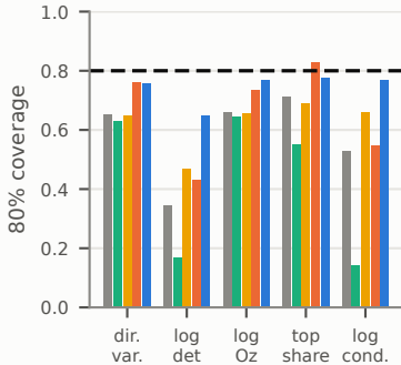
(b) Calibration, split-half
