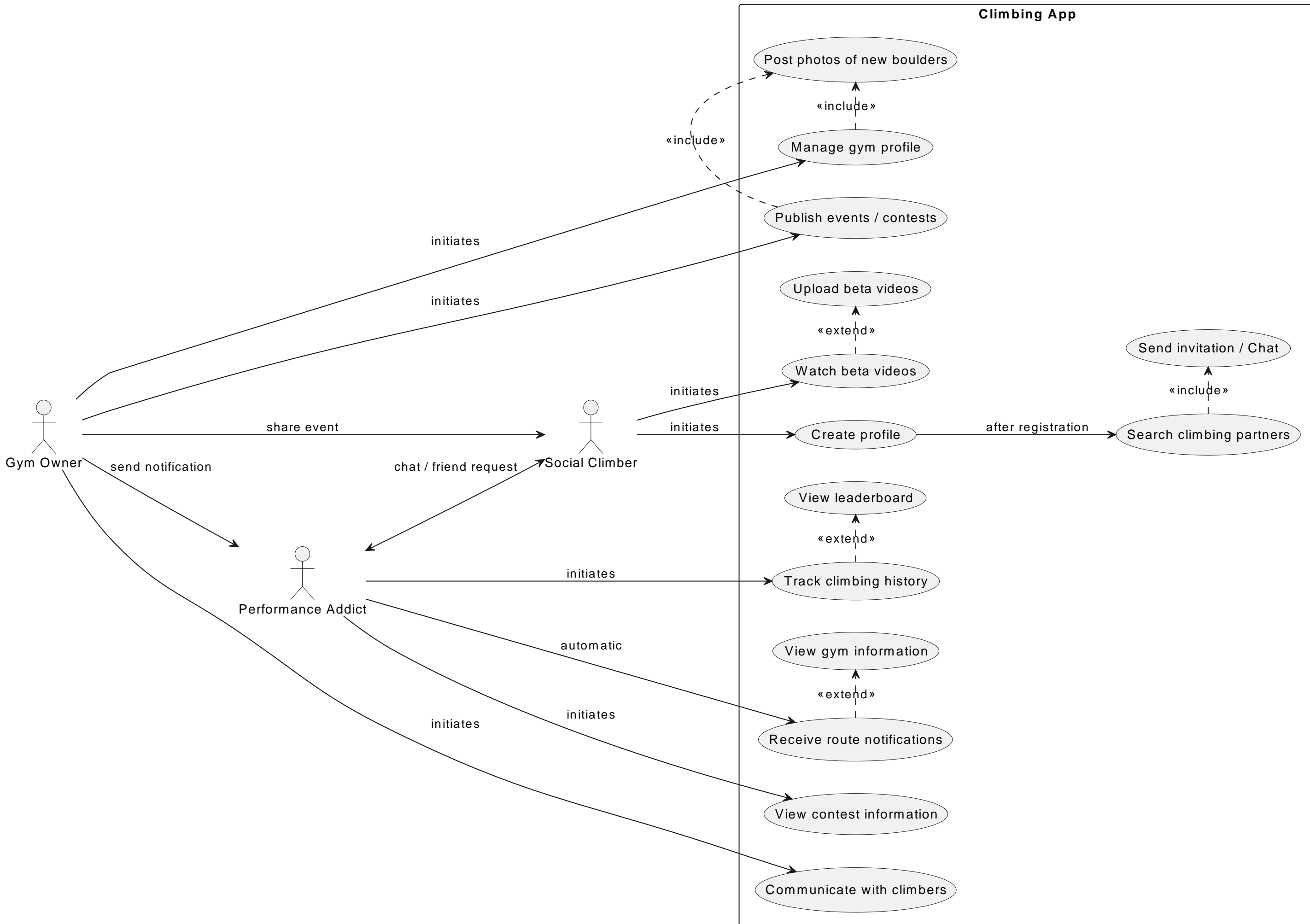
Climbing App - Use Case Diagram
