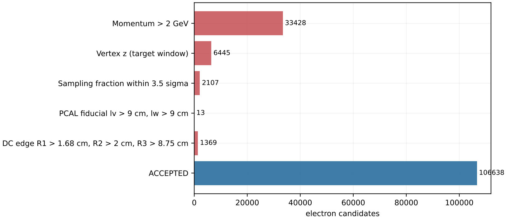
Electron selection: where candidates are lost
