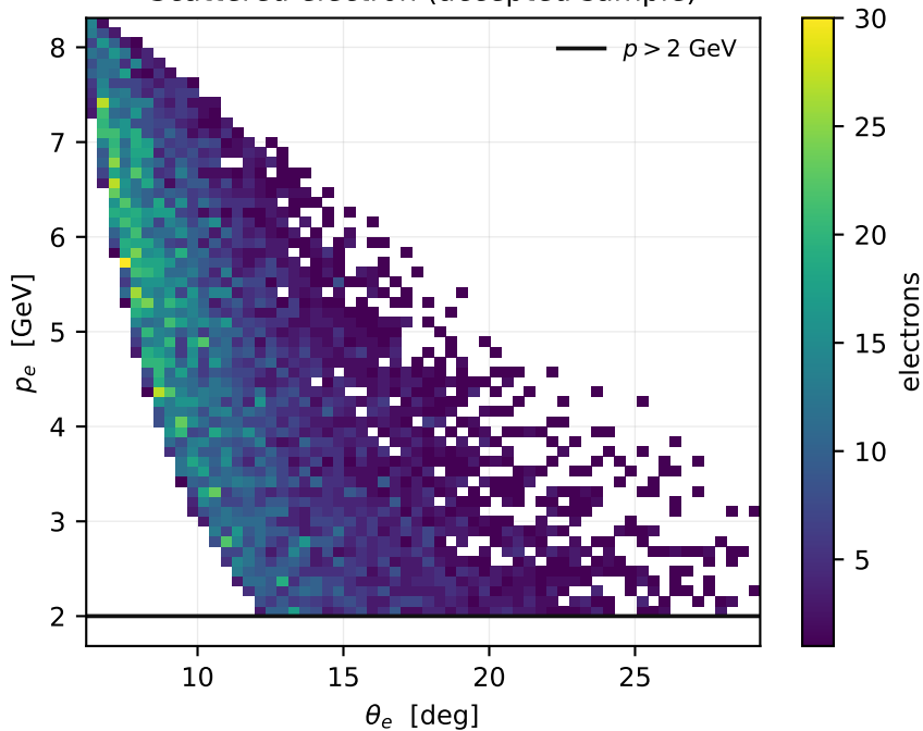
Scattered electron (accepted sample)
