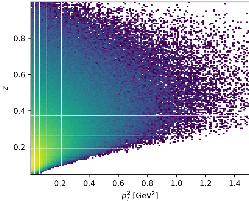
Grid B ( p_T^2, z )
