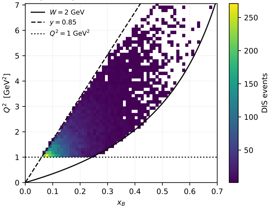
DIS phase space, with the selection boundaries
