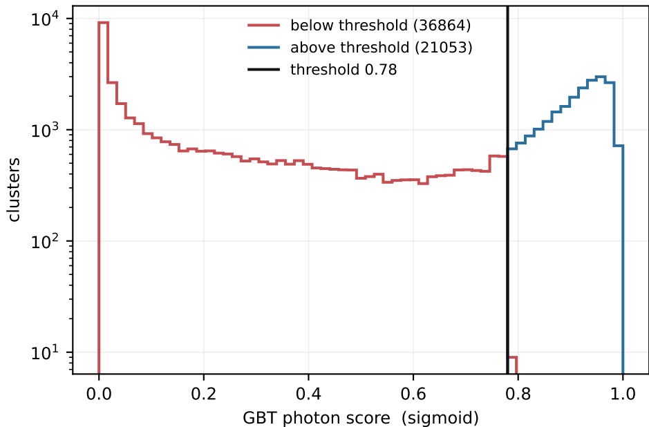
Photon identification — 23598 clusters pre-filtered, never scored
