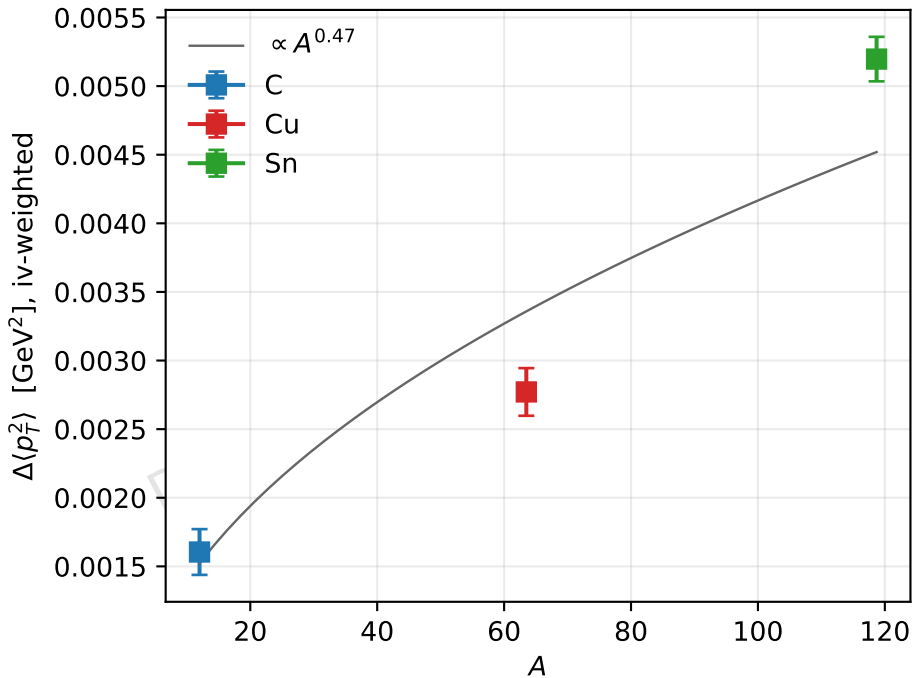
p_T broadening vs A
