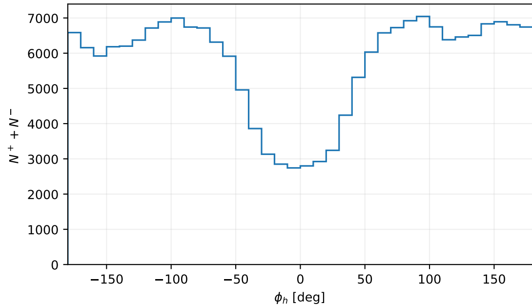
\phi_h yield, LD 2 (raw acceptance)
