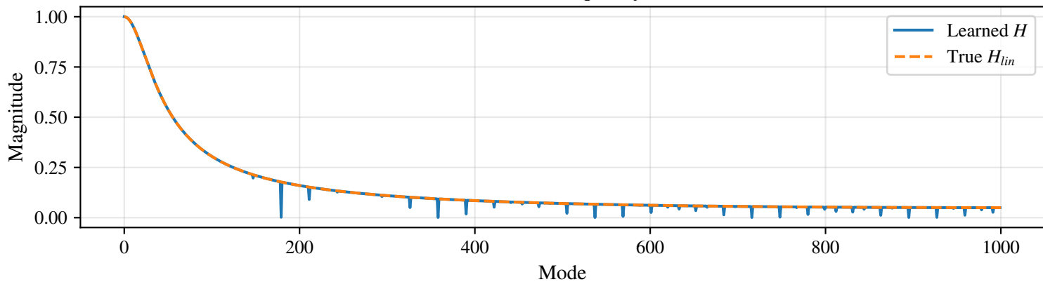
Learned kernel (Frequency domain)
