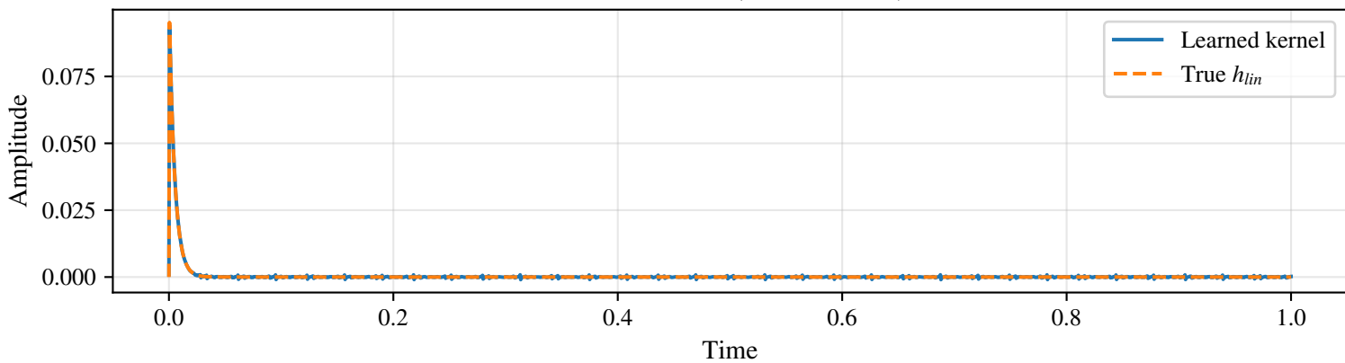
Learned kernel (Time domain)
