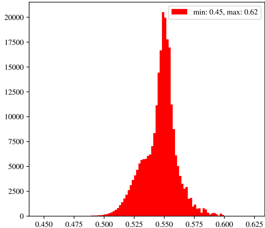
Target Distribution
