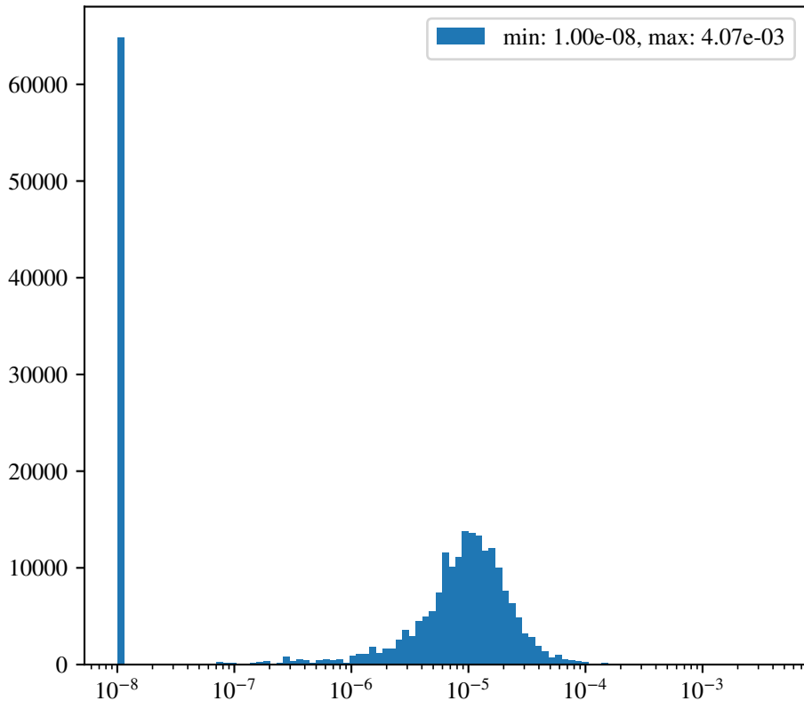
Feature Distribution
