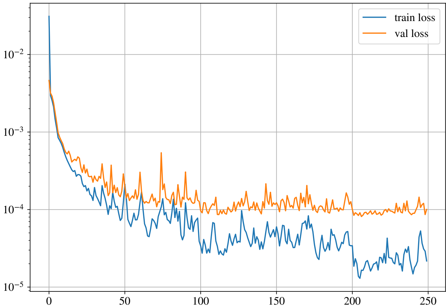
Loss History
