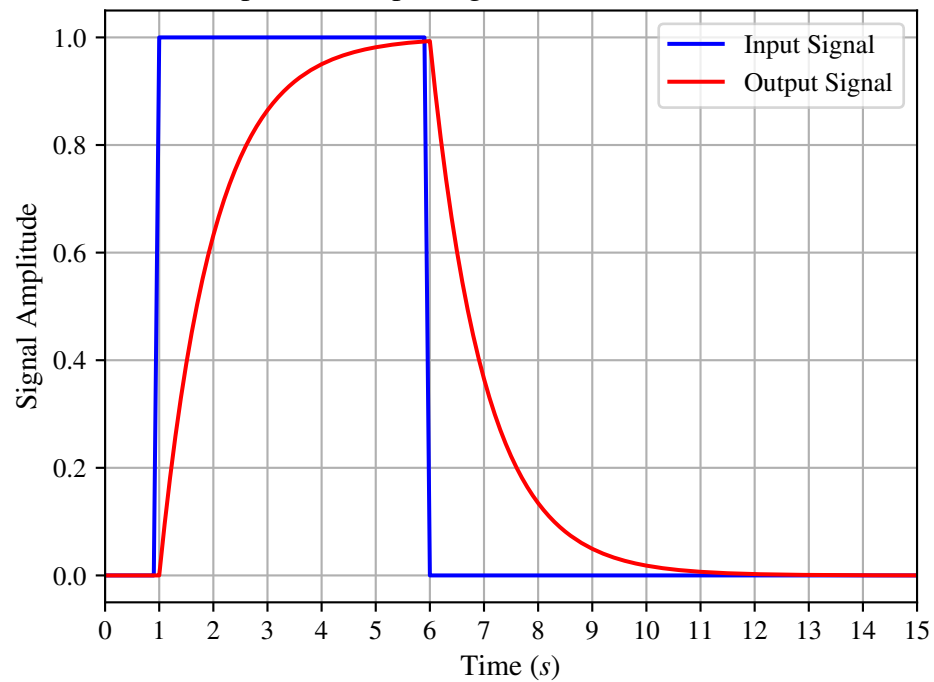
Input and Output Signals Over Time (ZOOM)
