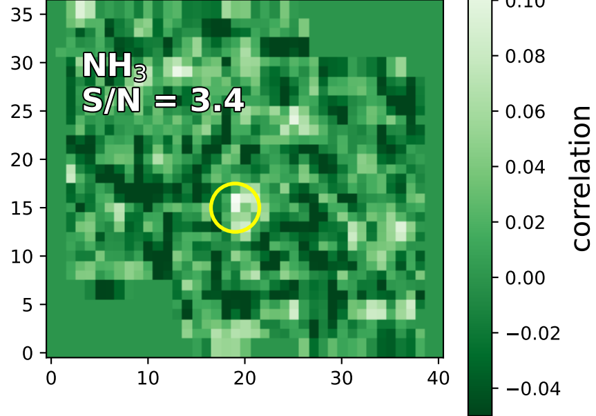
Band 2C : 10.0 - 11.7 \mu\text{m}
