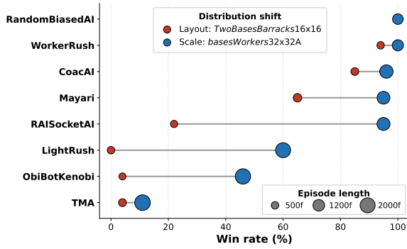
Fig. 6. UECD-Best Generalization Probes: layout vs scale shifts.
