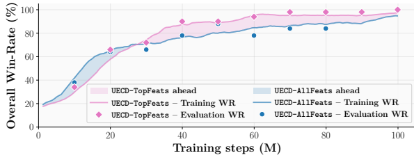
Fig. 2. Training Curves: WRs of UECD-TopFeats vs UECD-AllFeats.
