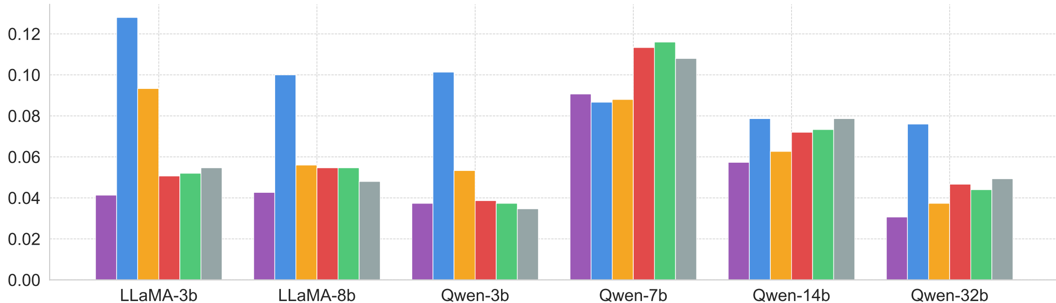
Post-Discussion Sycophancy Rate
