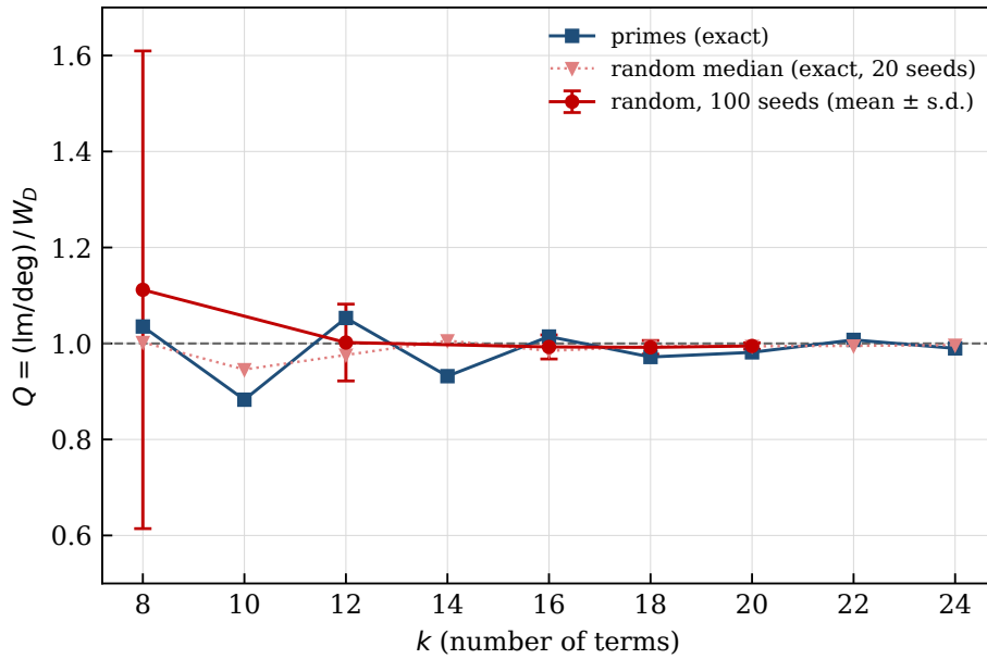
Figure 2: Convergence of Q = (\text{lm} / \deg) / W_D . Error bars are one standard deviation over 100 random sequences; they contract steadily, consistent with \varepsilon \rightarrow 0 . The primes (blue) oscillate about 1 rather than converging monotonically; see §8.4 and Conjecture 10.6.
