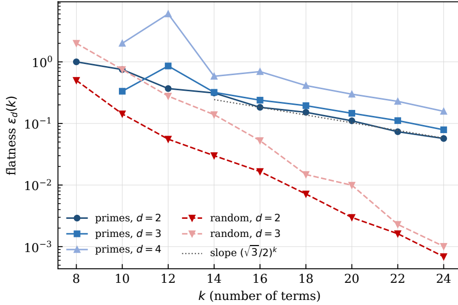
Figure 1: Exact flatness \varepsilon_d(k) on a logarithmic scale. The primes (blue) track the reference slope (\sqrt{3}/2)^k predicted by the modulo-6 heuristic of §7.3(i); random odd sequences (red, median over 20 seeds) decay strictly faster.
