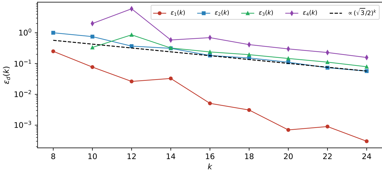
Measured flatness \varepsilon_d(k) for the primes against the mod-6 rate (\sqrt{3}/2)^k
