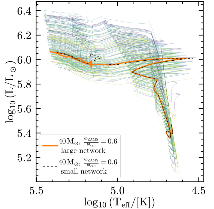
Figure 2. Hertzsprung-Russel diagram of rotationally-induced chemically-homogeneous evolving single star models. Dark (light) colors correspond to lower (higher) initial rotation rates. The orange thick line marks a representative 40 M_{\odot} , \omega_{\text{ZAMS}} = 0.6 \omega_{\text{crit}} used in O. Gottlieb et al. (2024), and the thin black dot-dashed line shows an otherwise identical model computed with only 22-isotopes from M. Renzo et al. (2024).
