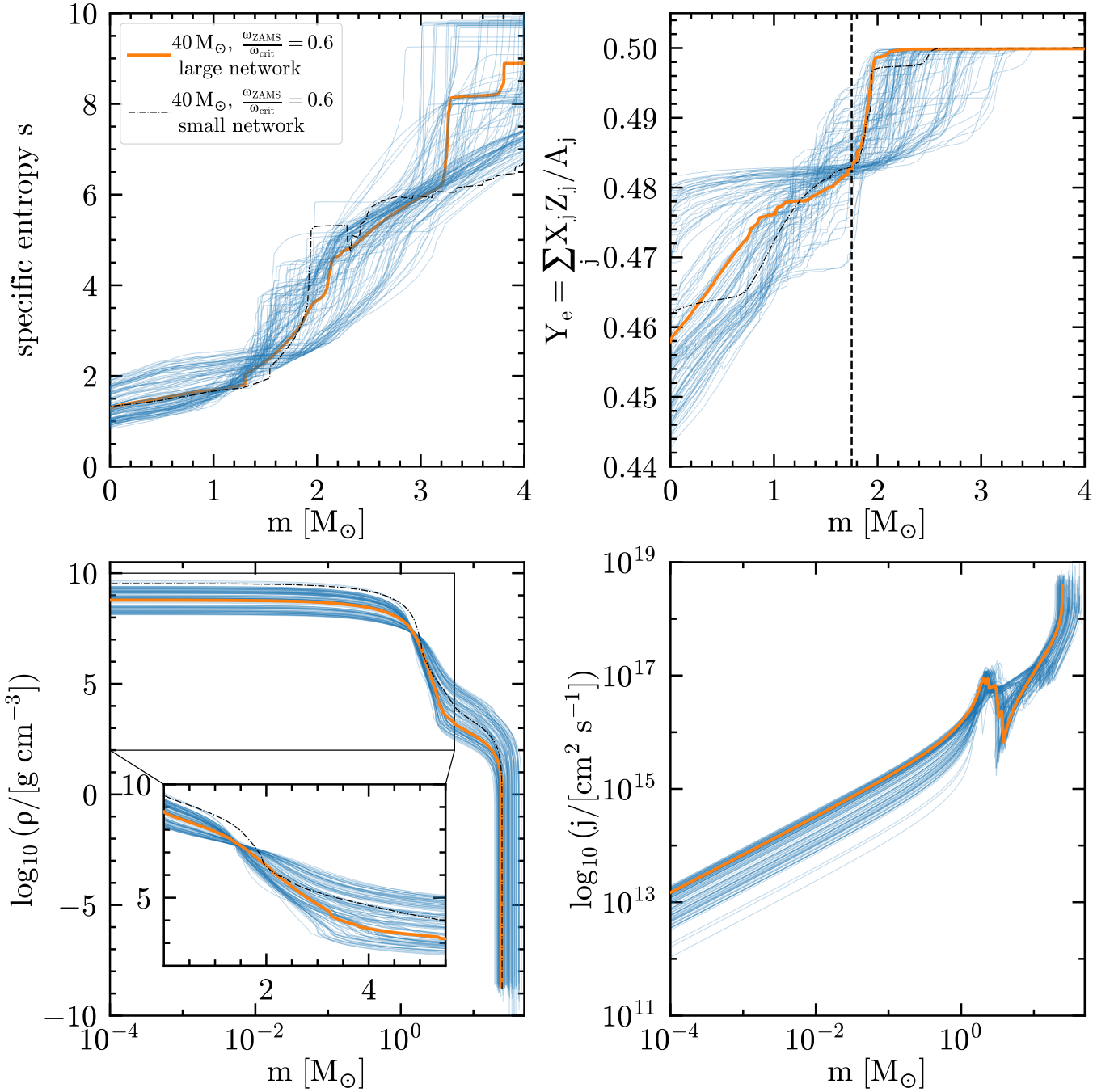
Figure 3. Top left: Inner specific entropy profiles. The dashed black horizontal line marks the s = 4 k_B N_A location often used in “explodability” criteria (e.g., T. Ertl et al. 2016; T. Ertl et al. 2020). Top right: Inner electron fraction Y_e(m) profile as a function of mass. The vertical dashed line marks \mathcal{M} = 1.75 M_\odot used to calculate the compactness \xi_{1.75} . Bottom left: Density profiles as a function of Lagrangian mass coordinate m on a logarithmic scale. The inset zooms on the inner region and uses a linear scale. Bottom right: Specific angular momentum profiles as a function of m . In all panels, the orange thick line marks a representative 40 M_\odot, \omega_{\text{ZAMS}} = 0.6 \omega_{\text{crit}} used in O. Gottlieb et al. (2024), and the thin black dot-dashed line shows an otherwise identical model computed with only 22-isotopes from M. Renzo et al. (2024).
