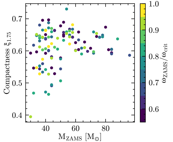
Figure 5. Compactness as a function initial mass and rotation rate for single CHE models.
