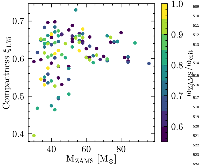
Figure 5. Compactness as a function initial mass and rotation rate for single CHE models. Higher values of compactness \xi_{\mathcal{M}} favor BH formation, but this does not imply without outflows and/or electromagnetic transients (e.g., A. Burrows et al. 2025; H.-S. Chan et al. 2026).
