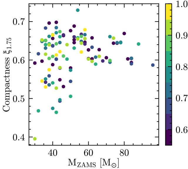
Figure 5. Compactness as a function initial mass and rotation rate for single CHE models. Higher values of compactness \xi_{\mathcal{M}} favor BH formation, but this does not imply without outflows and/or electromagnetic transients (e.g., A. Burrows et al. 2025; H.-S. Chan et al. 2026).
