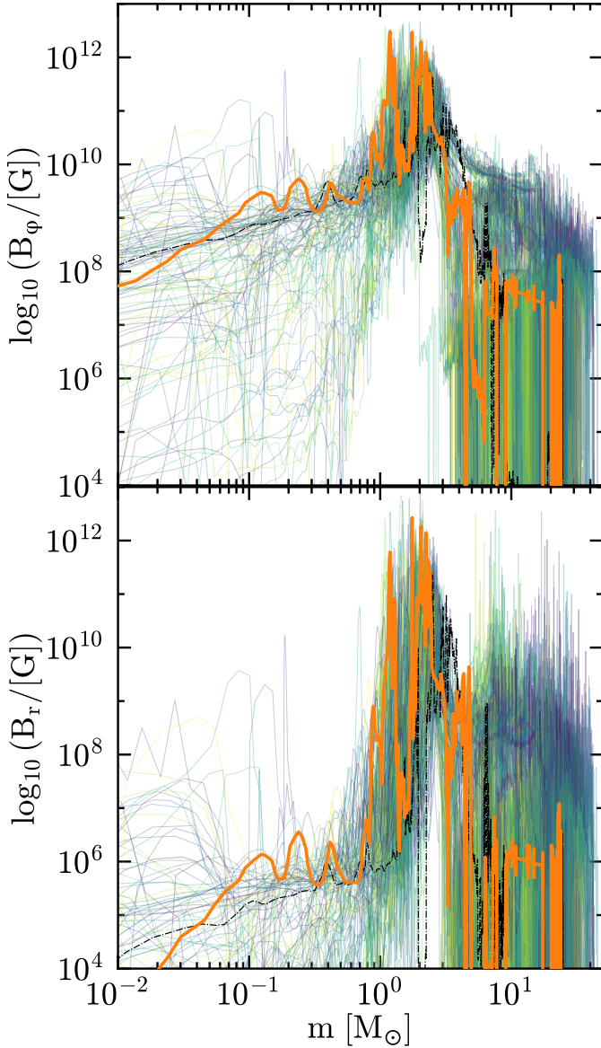
Figure 4. Azimuthal (top) and radial (bottom, local) component of the magnetic field generated by the Tayler-Spruit dynamo as a function of Lagrangian mass coordinate. Dark (light) colors correspond to lower (higher) initial rotation rates. The orange thick line shows the 40M_{\odot} , \omega_{\text{ZAMS}} = 0.6\omega_{\text{crit}} model from O. Gottlieb et al. (2024) and the thin black dot-dashed line shows an otherwise identical model computed with only 22-isotopes from M. Renzo et al. (2024).
