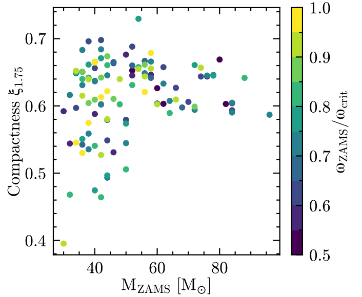
Figure 5. Compactness as a function of initial mass and rotation rate for single CHE models. Higher values of compactness \xi_{\mathcal{M}} favor BH formation, but this does not imply without outflows and/or electromagnetic transients (e.g., A. Burrows et al. 2025; H.-S. Chan et al. 2026).
