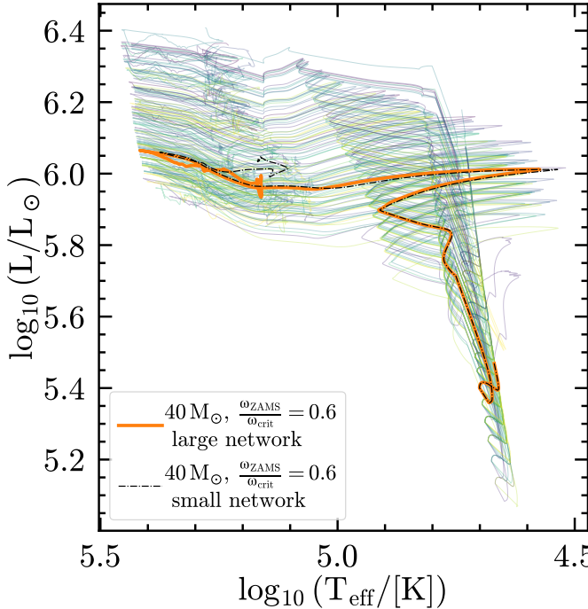
Figure 2. Hertzsprung-Russell diagram of rotationally-induced chemically-homogeneous evolving single star models. Dark (light) colors correspond to lower (higher) initial rotation rates. The orange thick line marks a representative 40 M_{\odot} , \omega_{\text{ZAMS}} = 0.6 \omega_{\text{crit}} used in O. Gottlieb et al. (2024), and the thin black dot-dashed line shows an otherwise identical model computed with only 22-isotopes from M. Renzo et al. (2024).
