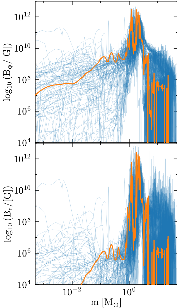
Figure 4. Azimuthal (top) and radial (bottom) component of the local magnetic field generated by the Spruit-Tayler dynamo as a function of Lagrangian mass coordinate. The orange thick line shows the 40M_{\odot} , \omega_{\text{ZAMS}} = 0.6\omega_{\text{crit}} model from O. Gottlieb et al. (2024).
