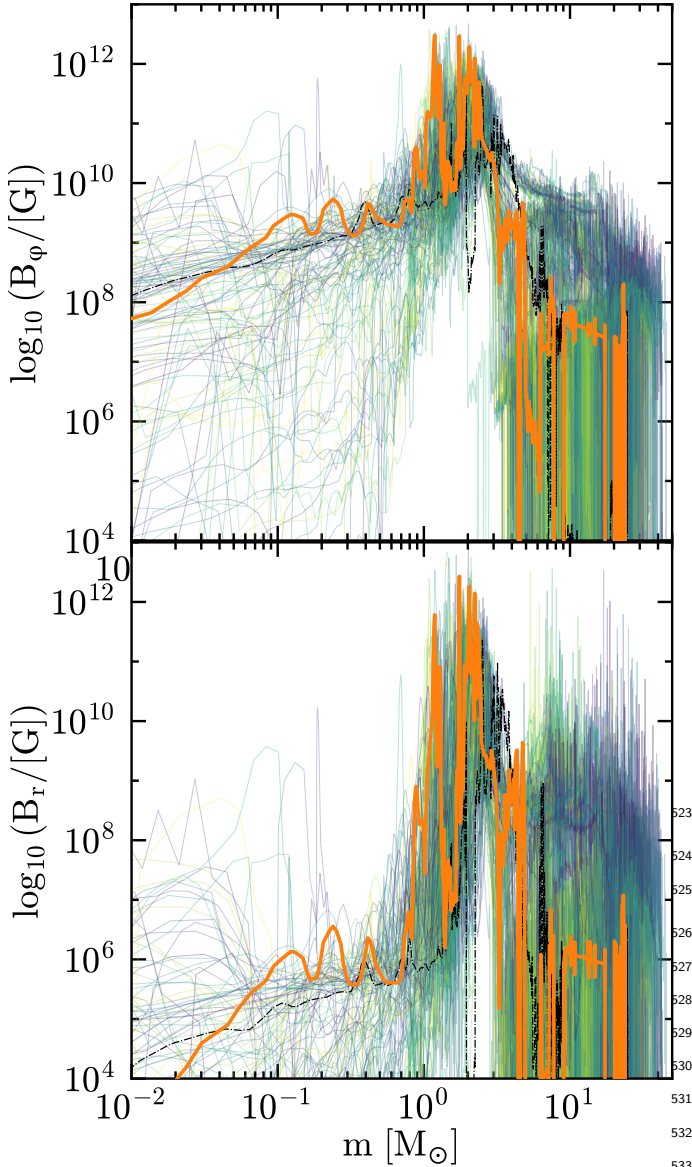
Figure 4. Azimuthal (top) and radial (bottom, local) component of the magnetic field generated by the Spruit-Taylor dynamo as a function of Lagrangian mass coordinate. The orange thick line shows the 40M_{\odot} , \omega_{\text{ZAMS}} = 0.6\omega_{\text{crit}} model from O. Gottlieb et al. (2024).
