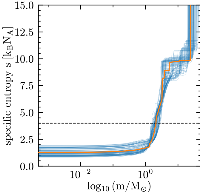
Figure 3. Specific entropy profiles. The dashed black horizontal line marks the s = 4 k_B N_A location often used in “explodability” criteria (e.g., T. Ertl et al. 2016; T. Ertl et al. 2020). The orange thick line shows the 40 M_\odot , \omega_{\text{ZAMS}} = 0.6 \omega_{\text{crit}} model from O. Gottlieb et al. (2024).
