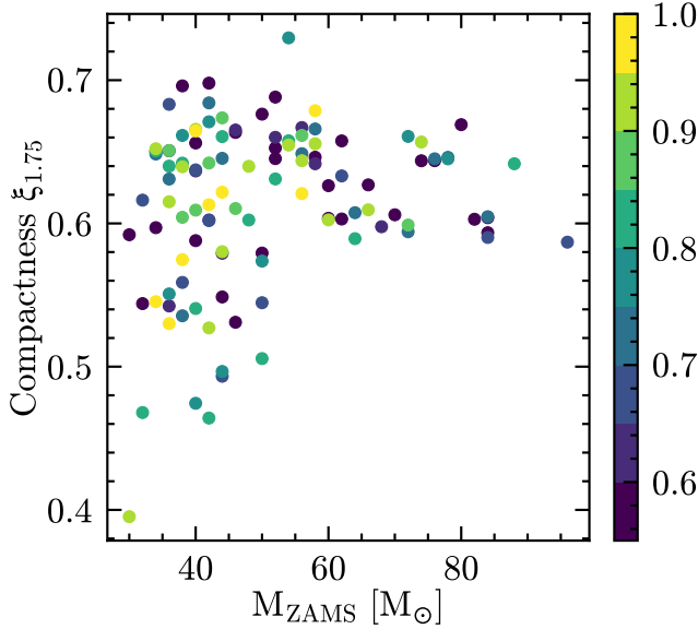
Figure 5. Compactness as a function initial mass and rotation rate for single CHE models.
