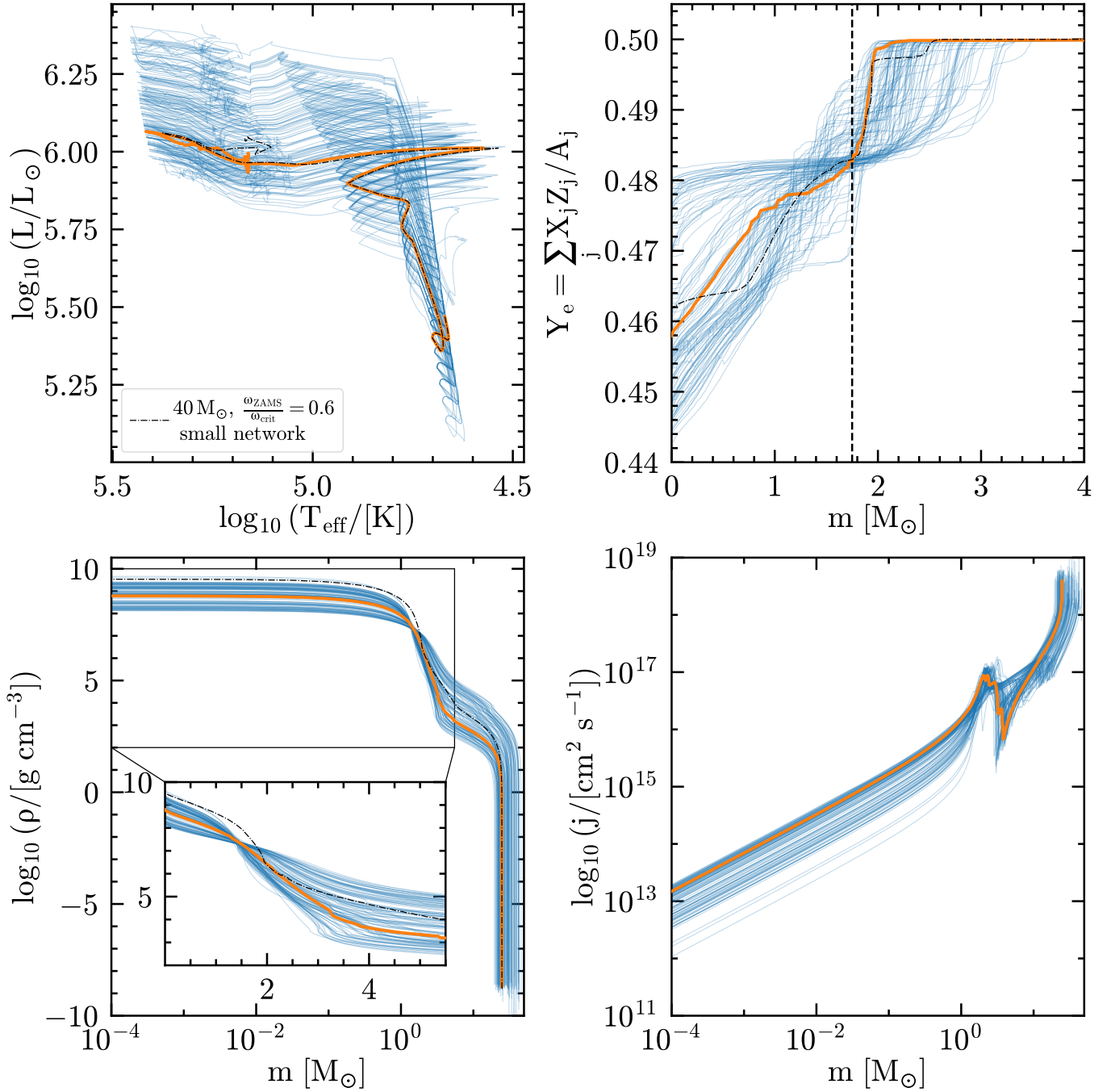
Figure 2. Top left: Hertzsprung-Russell diagram of rotationally-induced chemically-homogeneous evolving single star models. Top right: Inner electron fraction Y_e(m) profile as a function of mass. The vertical dashed line marks \mathcal{M} = 1.75 M_{\odot} used to calculate the compactness \xi_{1.75} . Bottom left: Density profiles as a function of Lagrangian mass coordinate m on a logarithmic scale. The inset zooms on the inner region and uses a linear scale. Bottom right: Specific angular momentum profiles as a function of m . In all panels, the orange thick line marks a representative 40 M_{\odot} , \omega_{\text{ZAMS}} = 0.6 \omega_{\text{crit}} used in O. Gottlieb et al. (2024), and the thin black dot-dashed line shows an otherwise identical model computed with only 22-isotopes from M. Renzo et al. (2024).
