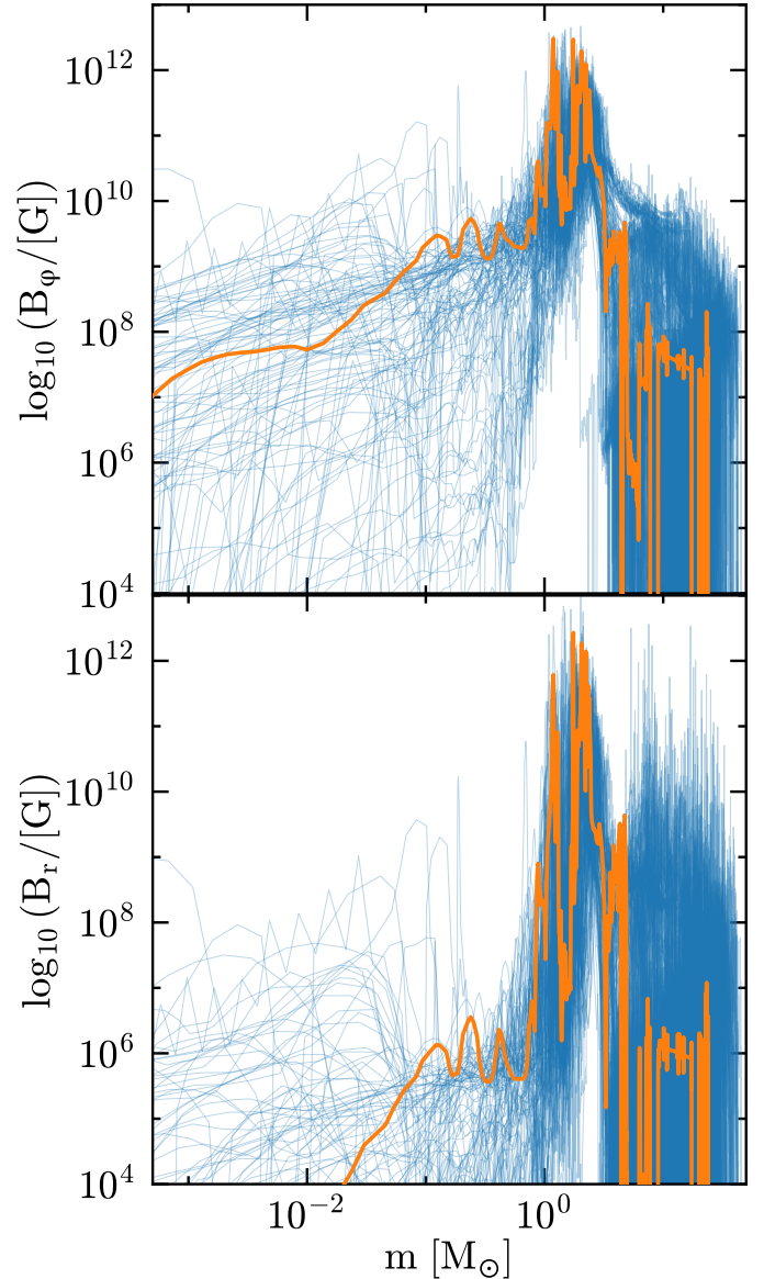
Figure 4. Azimuthal (top) and radial (bottom) component of the local magnetic field generated by the Spruit-Tayler dynamo as a function of Lagrangian mass coordinate. The orange thick line shows the 40 M_\odot , \omega_{\text{ZAMS}} = 0.6 \omega_{\text{crit}} model from O. Gottlieb et al. (2024).
