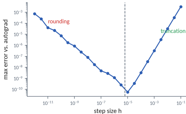
Figure 16. Error of the central difference against the step size h , for a small network. Rounding error dominates for small h and truncation error for large h ; the best h is near 10^{-5} .
