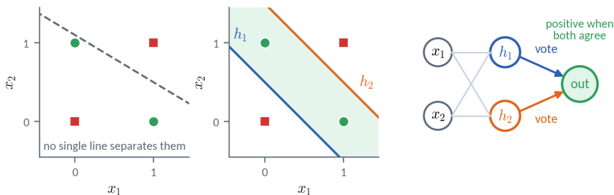
Figure 6. Exclusive or. Left: no single line separates the two classes. Middle: two hidden units each draw a line. Right: the output unit combines their votes and labels the band between the lines positive.
