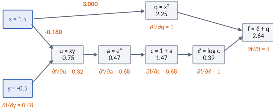
Figure 14. The backward pass for f(x, y) = \log(1 + e^{xy}) + x^2 at x = 1.5, y = -0.5 . Forward values are in blue and gradients in orange. The two uses of x send back -0.160 and 3.000 , which add to 2.840 .
