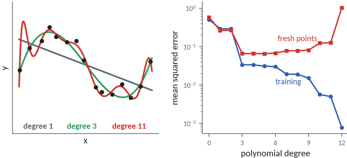
Figure 4. Overfitting. Left: polynomials of degree 1, 3, and 11 fitted to the same 15 noisy points from a sine curve. Right: as the degree grows, the error on the training points keeps falling, while the error on fresh points falls and then rises.
