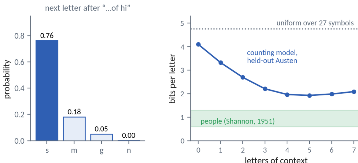
Figure 8. Shannon’s guessing game. Left: a counting model’s probabilities for the letter after “she could not help thinking of hi”. Right: bits per letter on held-out text as the counting model sees more letters of context, against the uniform baseline and Shannon’s estimate for people.
