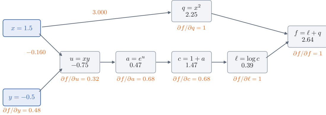
Figure 14. The backward pass for f(x, y) = \log(1 + e^{xy}) + x^2 at x = 1.5, y = -0.5 . Forward values are in blue and gradients in orange. The two uses of x send back -0.160 and 3.000 , which add to 2.840 .
