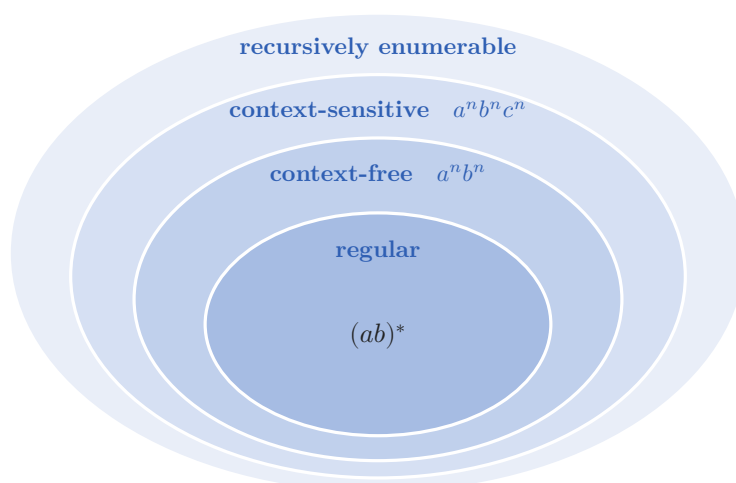
Figure 7. The Chomsky hierarchy. Each class of languages contains the ones inside it; the examples, strings of the form a...a\ b...b\ (c...c) with equal counts, need progressively more powerful grammars.
