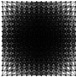
(h) 2026: unit distances in a rescaled square grid, the construction the new result beats
