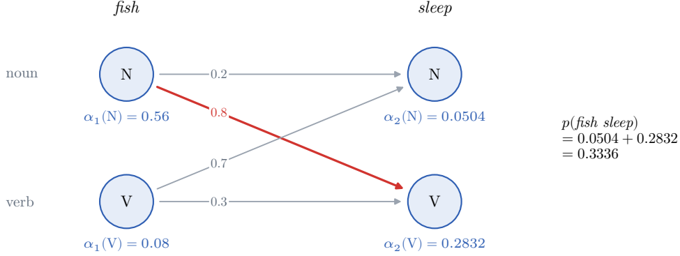
Figure 23. The forward algorithm on “fish sleep”. Each node holds \alpha_t , the probability of the words so far and the current state; edges carry transition probabilities. The red edge is the most probable path, N then V.
