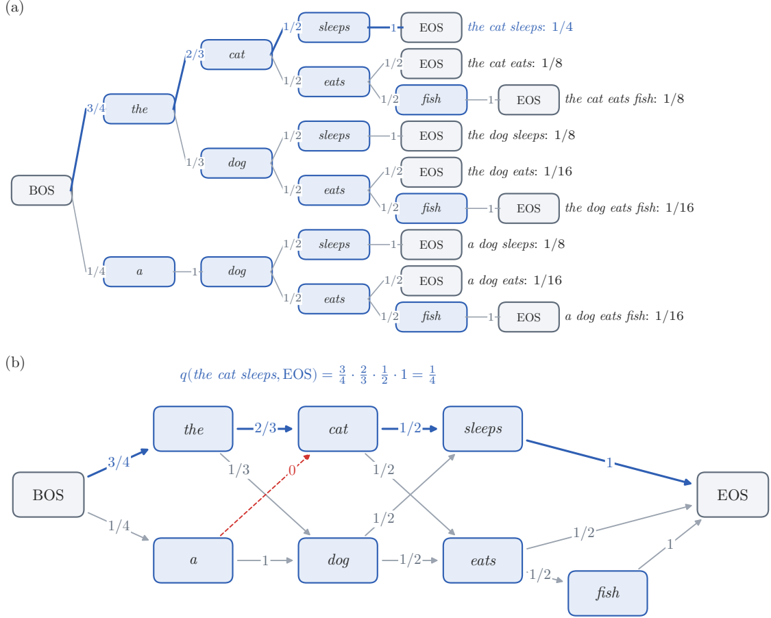
Figure 2. The bigram model of the four-sentence corpus. (a) As a tree of prefixes: every branch carries a maximum-likelihood probability q(w | h) , and every EOS leaf ends a complete sentence whose probability is the product along its path; the leaves sit at different depths because the sentences have different lengths, and the nine probabilities sum to one. (b) As a Markov chain: the tree’s nodes that end in the same word share their branch probabilities and are merged into one state. The blue path is “the cat sleeps”, with probability 1/4. The dashed red arrow, from “a” to “cat”, was never observed, so its probability is zero.
