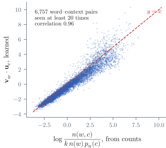
Figure 10. What skip-gram learned, against what counting predicts. Each point is a word–context pair from the TinyStories run that occurs at least 20 times. Horizontal: the shifted PMI that the argument above predicts, computed from the pair counts. Vertical: the dot product \mathbf{v}_w \cdot \mathbf{u}_c of the trained vectors. Points on the dashed diagonal are pairs where the vectors learned exactly what the counts predict; the correlation is 0.96.
