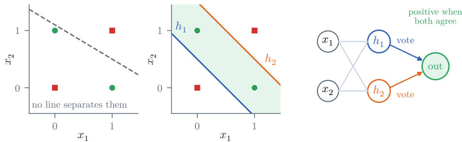
Figure 6. Exclusive or. Left: no single line separates the two classes. Middle: two hidden units each draw a line. Right: the output unit combines their votes and labels the band between the lines positive.
