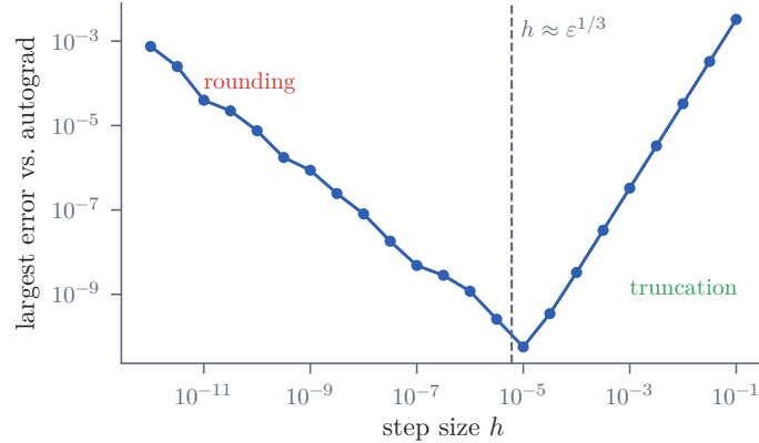
Figure 16. Error of the central difference against the step size h , for a small network. Rounding error dominates for small h and truncation error for large h ; the best h is near 10^{-5} .
