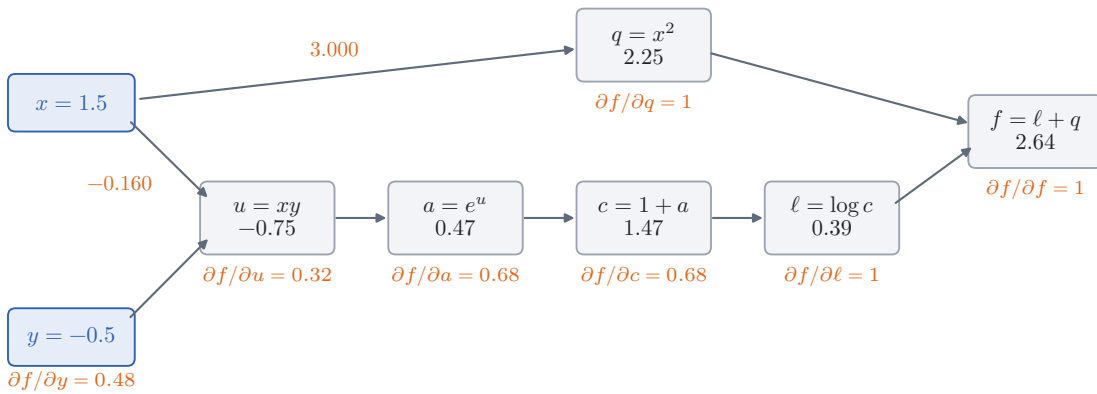
Figure 14. The backward pass for f(x, y) = \log(1 + e^{xy}) + x^2 at x = 1.5 , y = -0.5 . Forward values are in blue and gradients in orange. The two uses of x send back -0.160 and 3.000 , which add to 2.840 .
