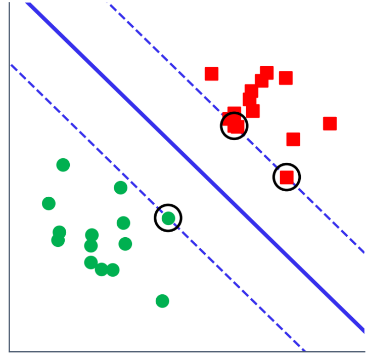
a maximum-margin classifier; the support vectors are circled
