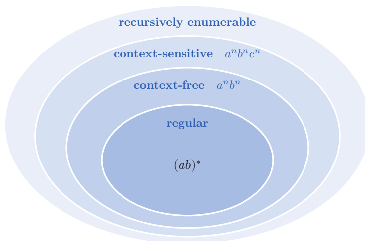
Figure 7. The Chomsky hierarchy. Each class of languages contains the ones inside it; the examples, strings of the form a \dots a b \dots b (c \dots c) with equal counts, need progressively more powerful grammars.
