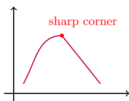
Graph A: Not smooth (sharp corner) \Rightarrow NOT a polynomial.
