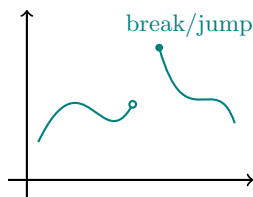
Graph C: Smooth pieces but discontinuous (jump) \Rightarrow NOT a polynomial.
