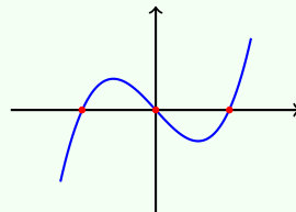
Cubic: 3 zeros, 2 turns
