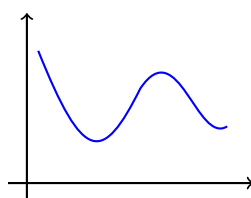
Graph B: Smooth and continuous \Rightarrow IS a polynomial.
