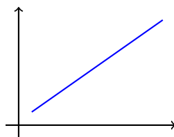
Graph D: A line — smooth and continuous \Rightarrow IS a polynomial (linear).
