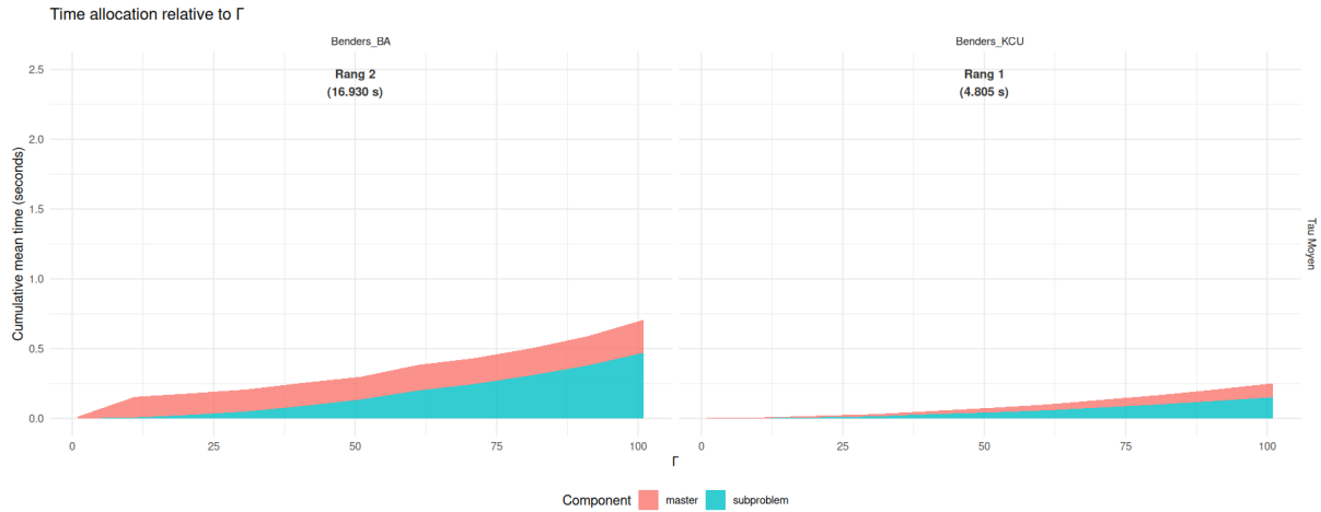
FIGURE 1 – Comparison of sub-problem and master problem times for BA & KCU.
