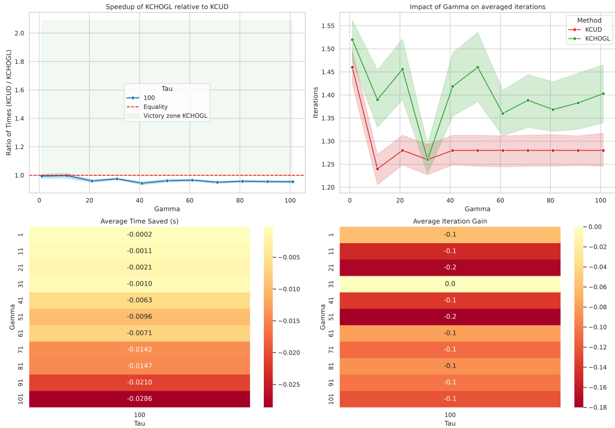
FIGURE 4 – Comparative analysis between KCUD &amp; KCHOGL.
