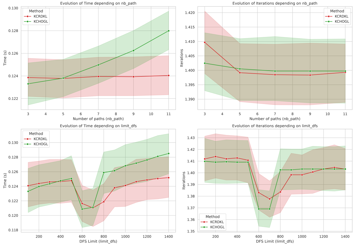
FIGURE 7 – Impact of N and L on performance.
