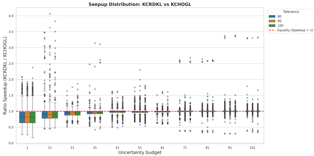
FIGURE 5 – Speedup distribution between KCRDKL & KCHOGL.
