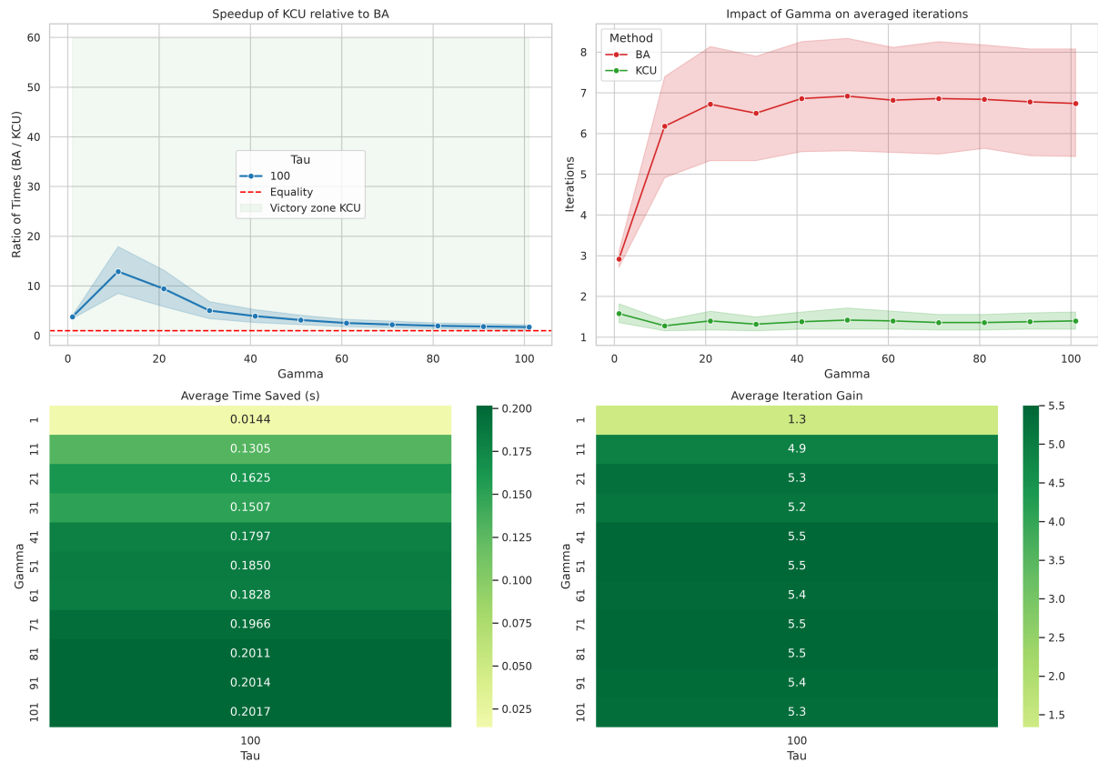
FIGURE 2 – Comparative analysis between BA & KCU.
