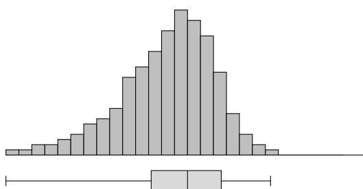
negatively skewed data ( n = 97 )
