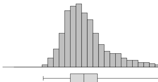
positively skewed data ( n = 134 )
