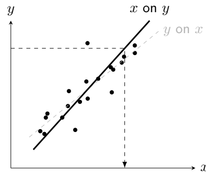
Prediction with an x on y model (Minimises squared horizontal distances)
