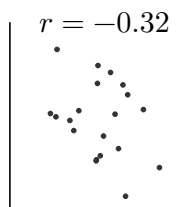
weak negative linear relationship
