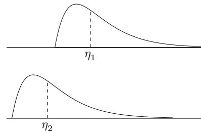
Different locations: \eta_1 \neq \eta_2
