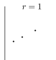
perfect positive linear relationship
