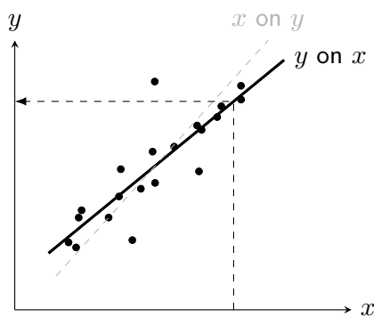
Prediction with a y on x model (Minimises squared vertical distances)
