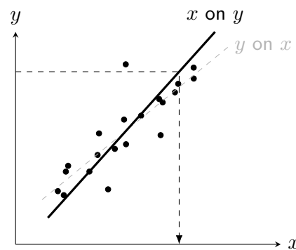
Prediction with an x on y model (Minimises squared horizontal distances)
